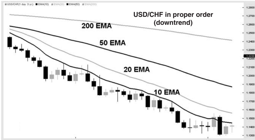
FIGURE 9.6 USD/CHF moving averages are in the “proper order” for a downtrend. Source: FXtrek IntelliChart™. Copyright © 2001–2006 FXtrek.com, Inc.
